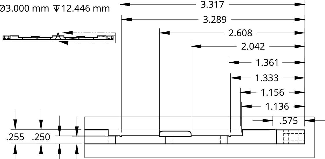
DETAIL A SCALE 2:2
